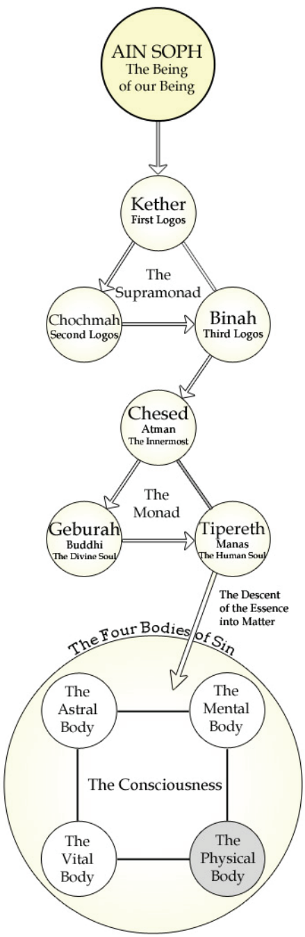
The Descending Ray of Creation as it relates with the number of Laws (left) and the manifestations of the Being (right).
